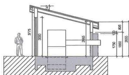
SNEYÐING X-X 1:100
