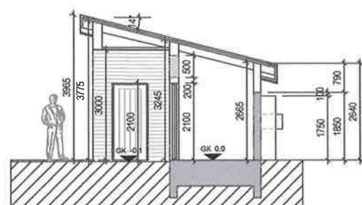
SNEYÐING Y-Y 1:100
